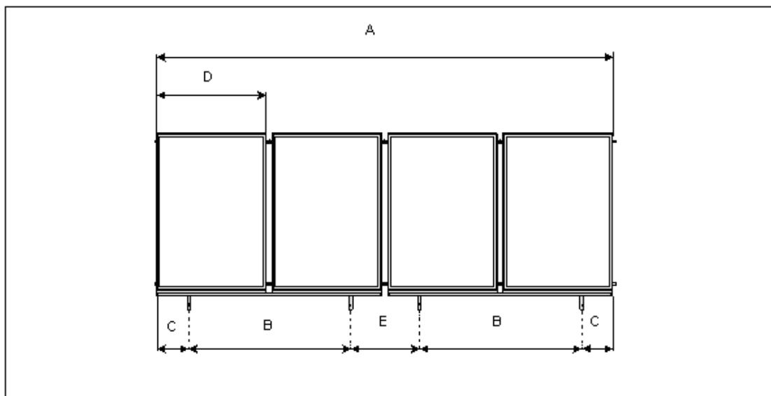
Figure 10. Bank of Four Solar Collectors
