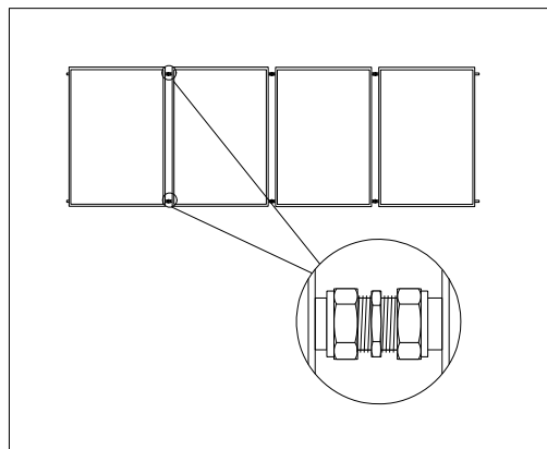
Figure5. Connections
