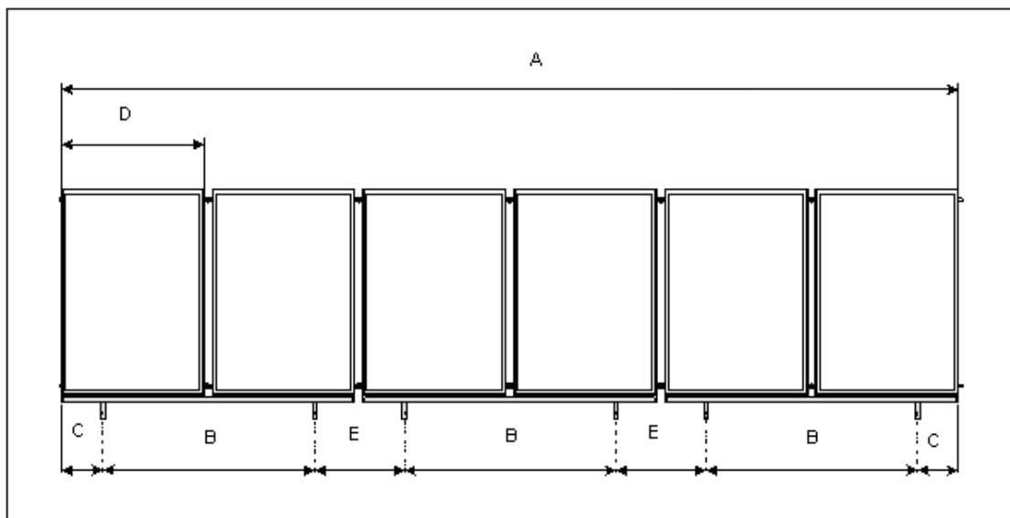
Figure 12. Bank of Six Solar Collectors
