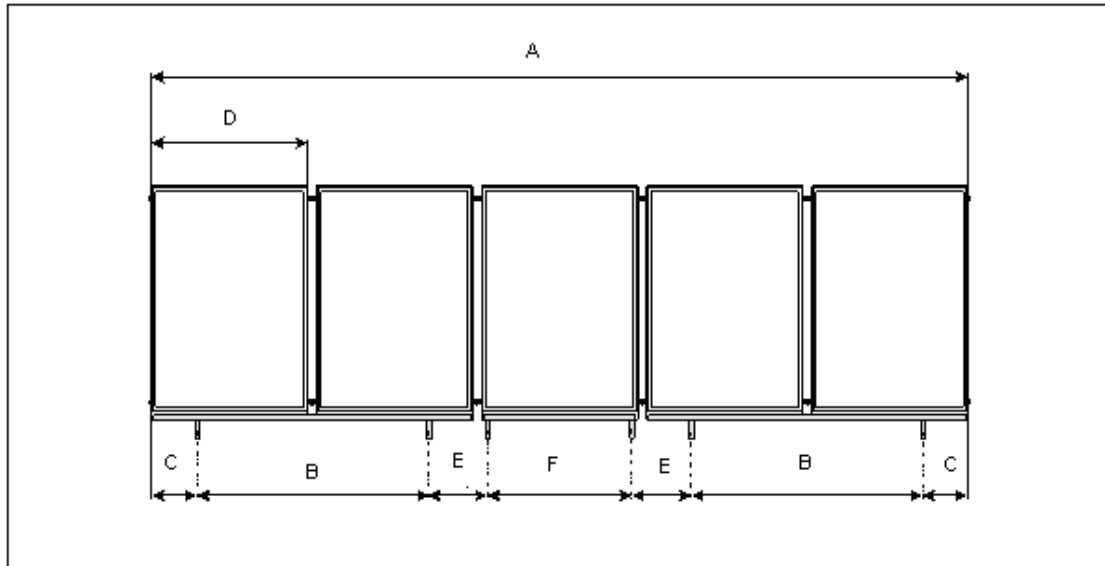
Figure 11. Bank of Five Solar Collectors
