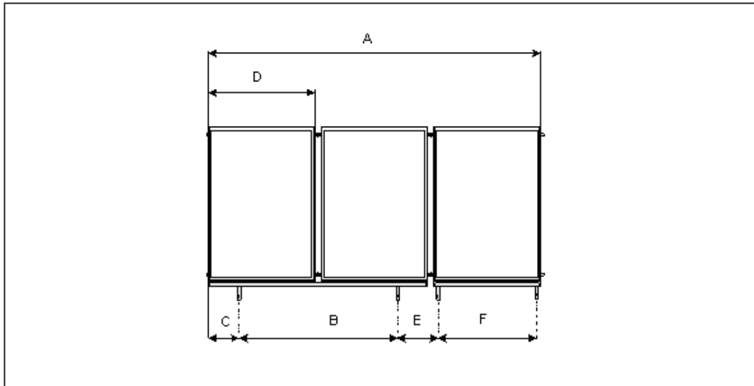
Figure 9. Bank of Three Solar Collectors
