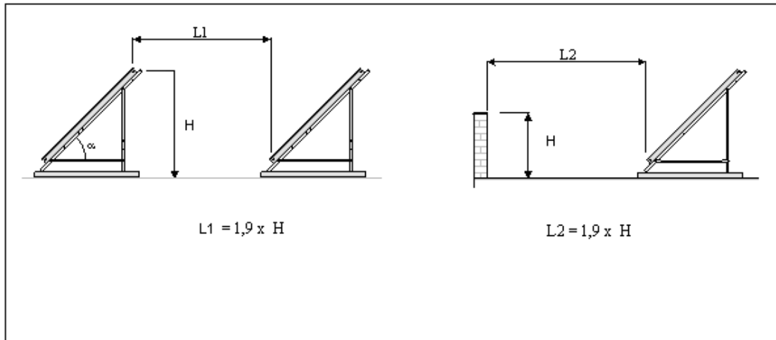
Figure 6. Distance needed in order to avoid shadows on collectors.
